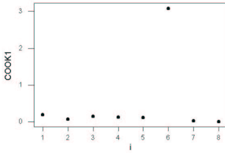
Cook's distance versus i
