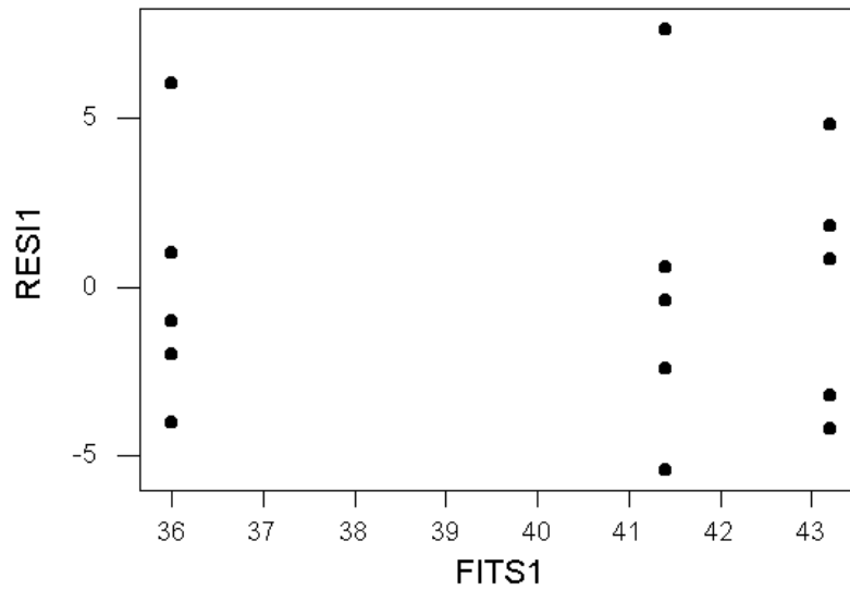
Residuals versus fitted values for one way model
