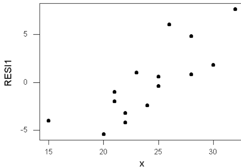
Residuals versus x values for one way model
