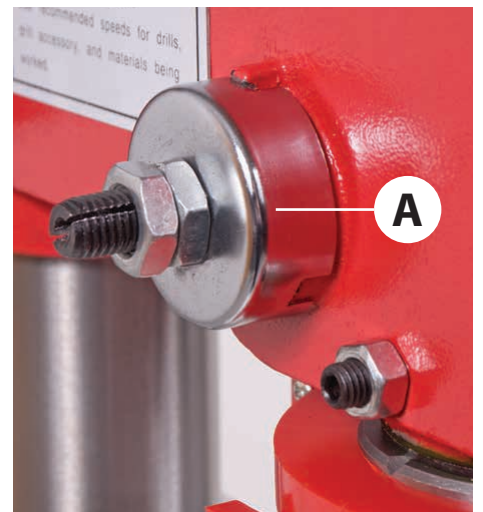
Quill rise and full return spring (A)
