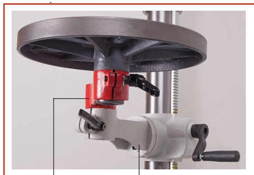
Extension arm Extension bracket arm
